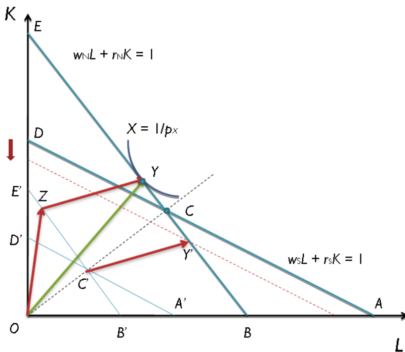
Figure 2. Fragmentation
