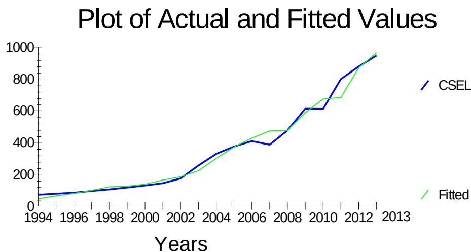
Figure 1E.19. Plot of Actual and Fitted Values of Electricity Demand in Commercial Sector
