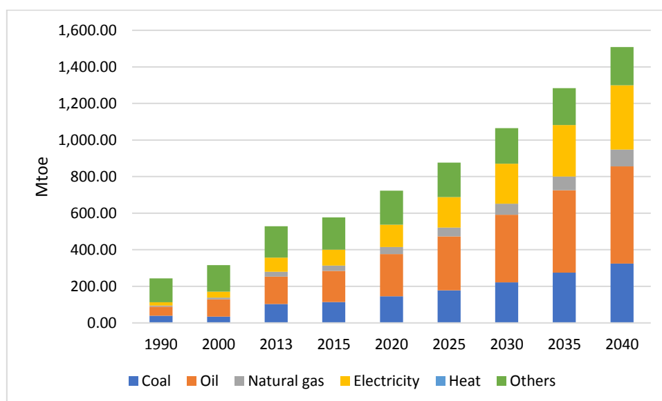
Figure 2C.3. Final Demand of Energy Sources in BAU
